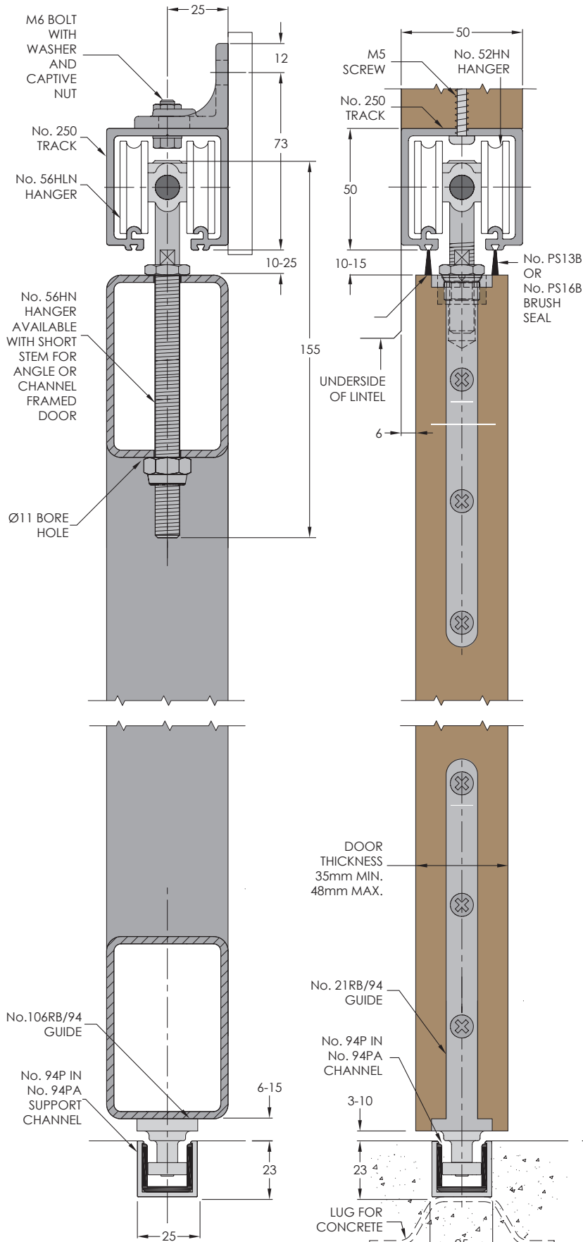
DOOR PREPARATION No. 52HN HANGER
